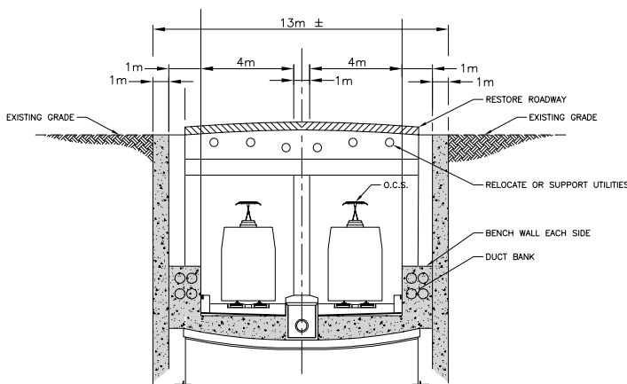
Prototypical Segment Type (Cut-and-Cover Tunnel)
