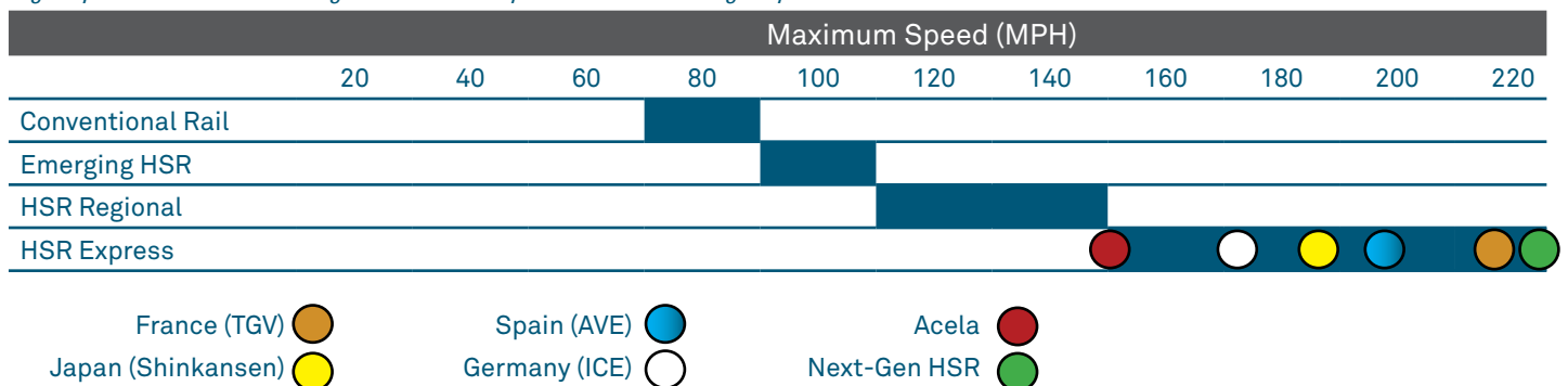
High-Speed Rail Service Categories and Examples of Next-Gen High-Speed Rail
